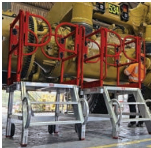
Handles for manoeuvrability, simply lift to engage the front wheels.
